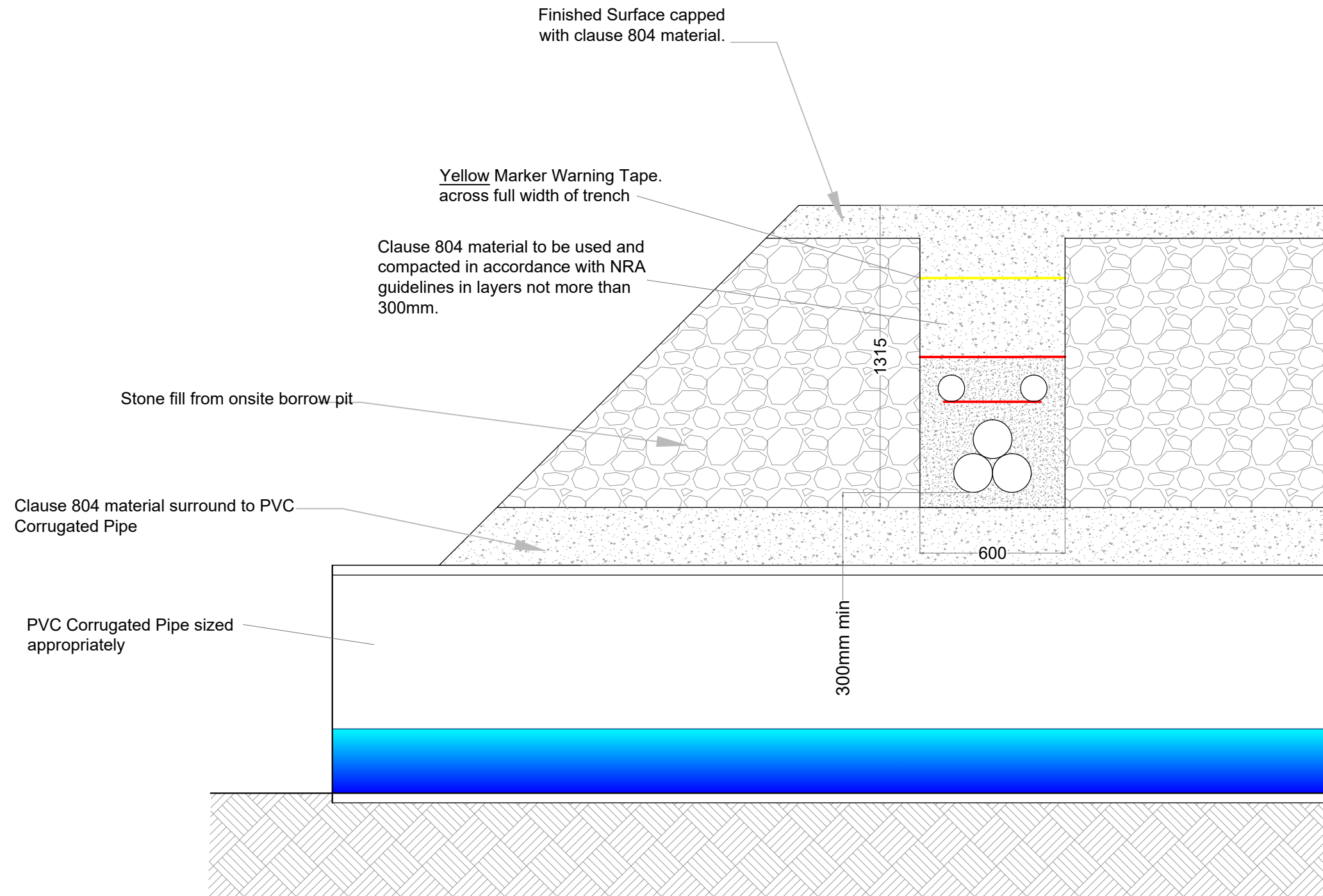
Option F - Pipe crossing - 110kV SCALE 1:20
